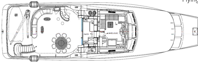
Bridge deck
