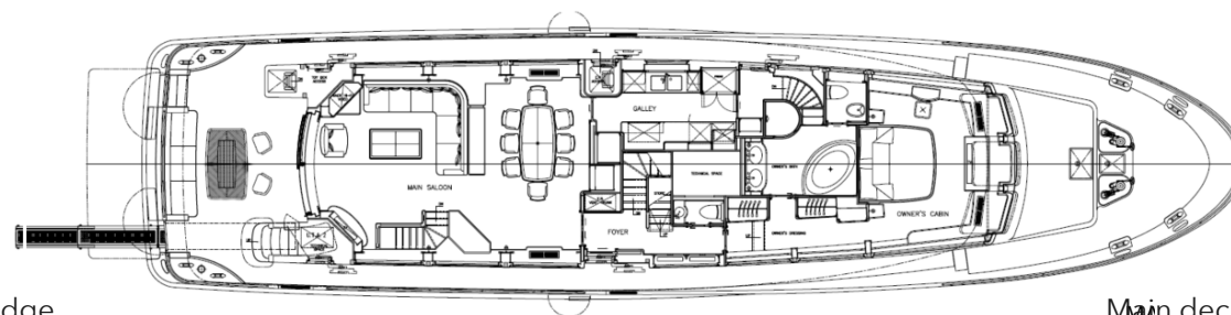
Flying bridge
