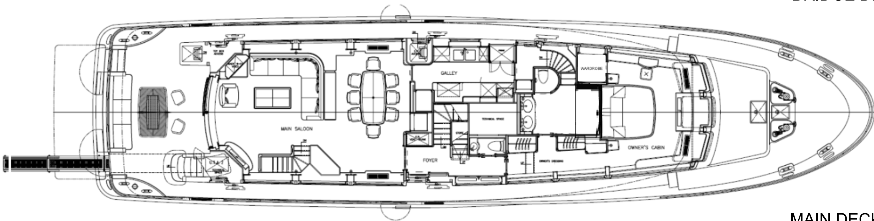
BRIDGE DECK
