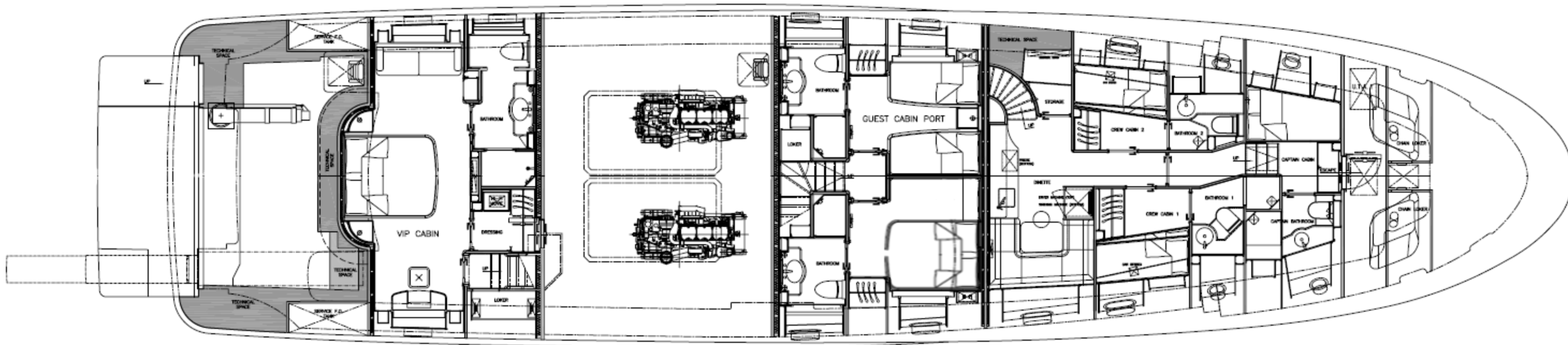
LOWER DECK
